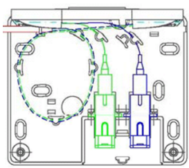
MCPE-02-SC A/SC S-A two SC pigtails
